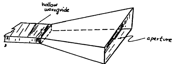
Horn Antenna
