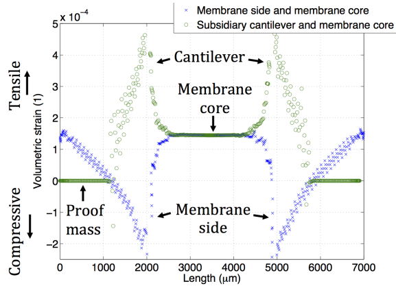
Figure 4: Strain distribution of the integrated cantilever membrane design for 100 g acceleration loading. The centre of the membrane experiences notable strain.
