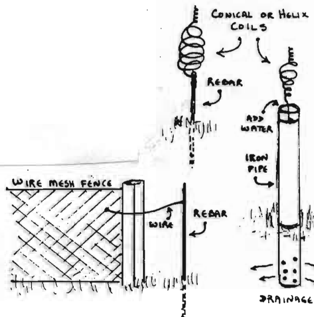
FIGURE 2: ANTENNA SYSTEMS
