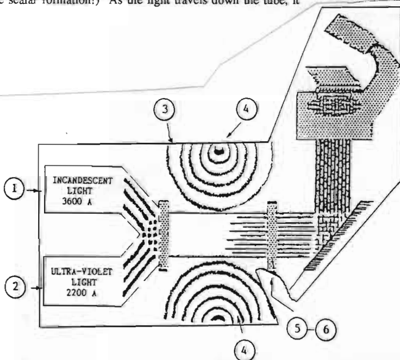
Two light sources, the first (1) an incandescent one with a wavelength of about 3600 angstrom, the second (2) an ultraviolet one with a wavelength of about 2200 angstrom beat against each other to produce a third wavelength of which passes through a monochromatic filter (3) to produce a monochromatic ray. This ray is exposed to magnetic fields (4)—the Zeeman effect—that divides it to produce numerous parallel rays (5) that, in turn pass through a Kerr cell (6) that increases the frequency. It is this light source, invisible to the naked eye, that strikes the specimen slides. The image is reconstituted by the microscope. Credit: Guide Resources
